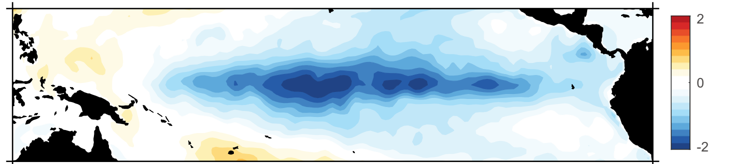
d 1975-76/1998-99/1999-2000 Dec-Feb SST anomaly
