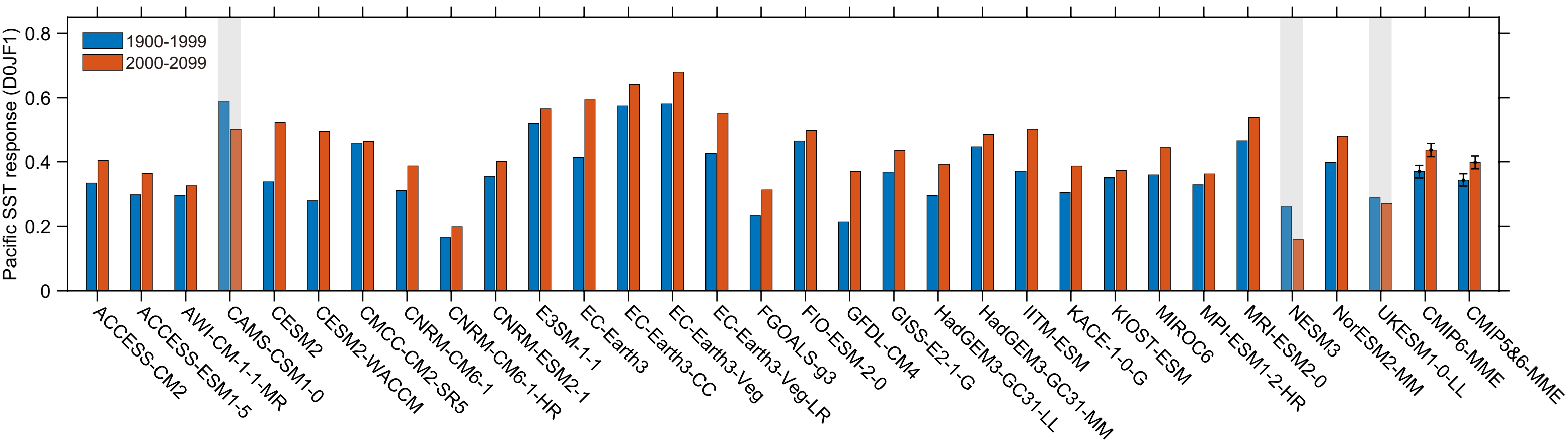
e Enhanced impact of NPMM forcing under future climate
