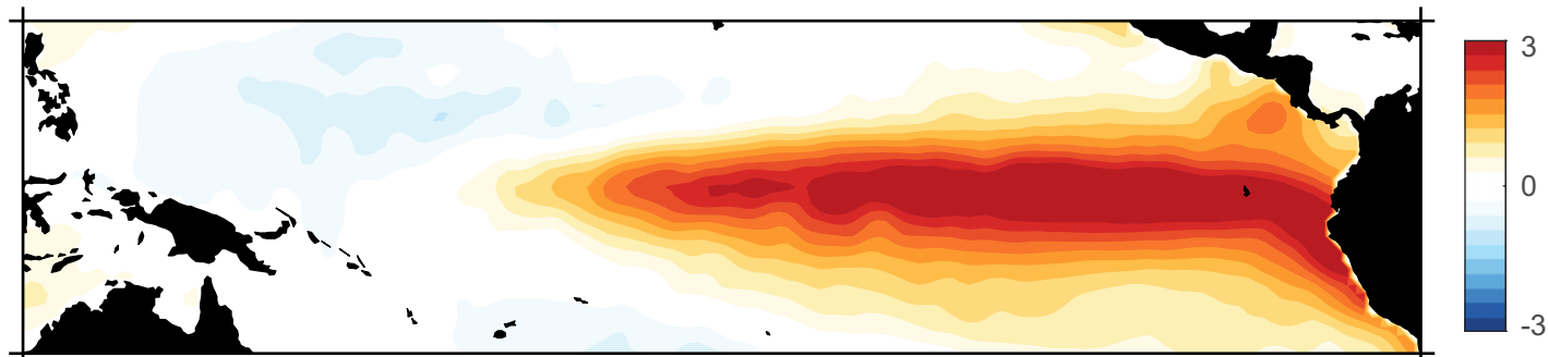
c 1982-83/1997-98/2015-16 Dec-Feb SST anomaly
